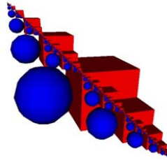
Figura 4. Octree infinito
